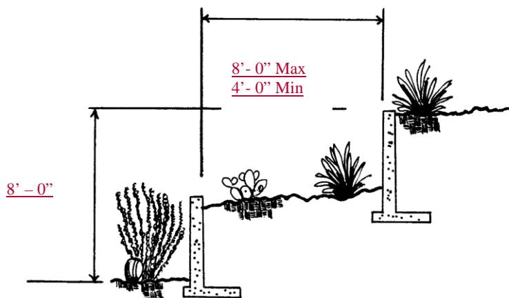
FIGURE 8 –TERRACED VERTICAL RETAINING WALLSRETAINING WALLS
