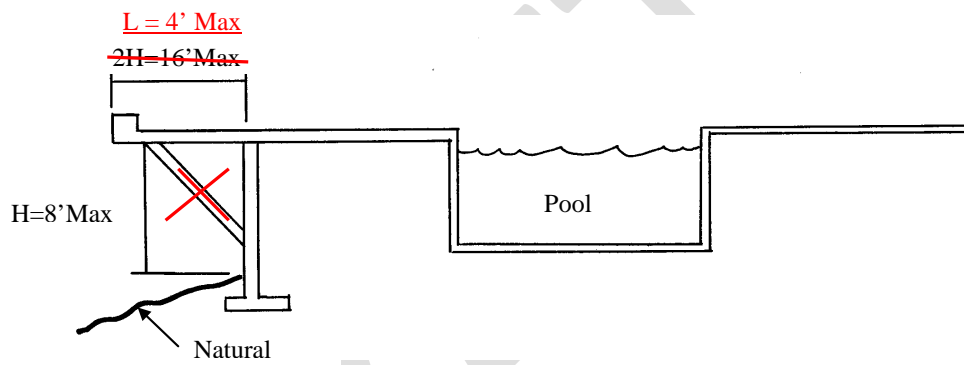
FIGURE 7 - HEIGHT FOR A CANTILEVERED ELEMENT
