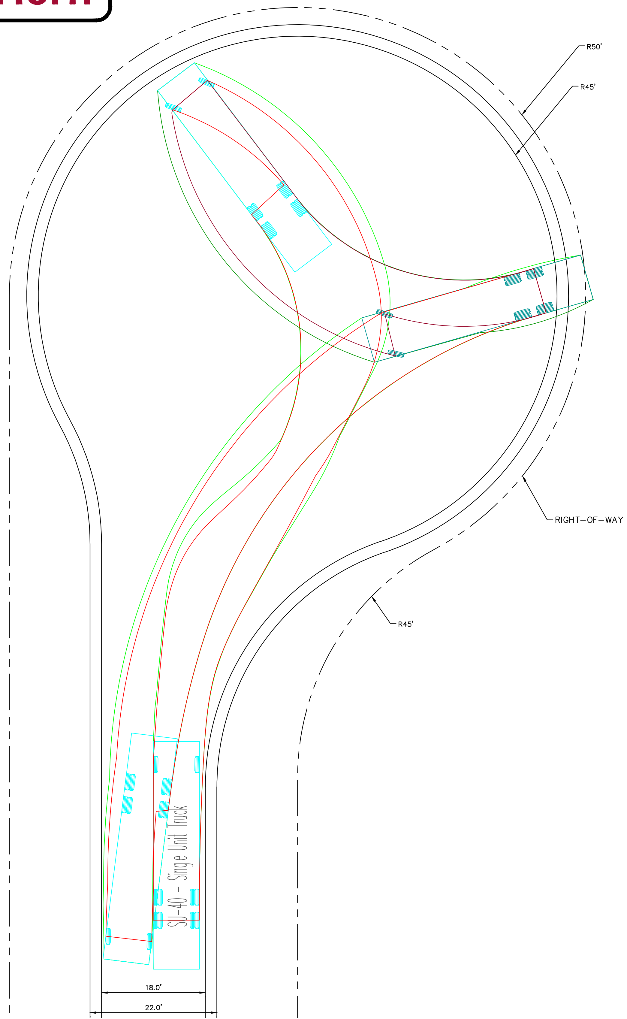
MODIFIED CUL-DE-SAC
