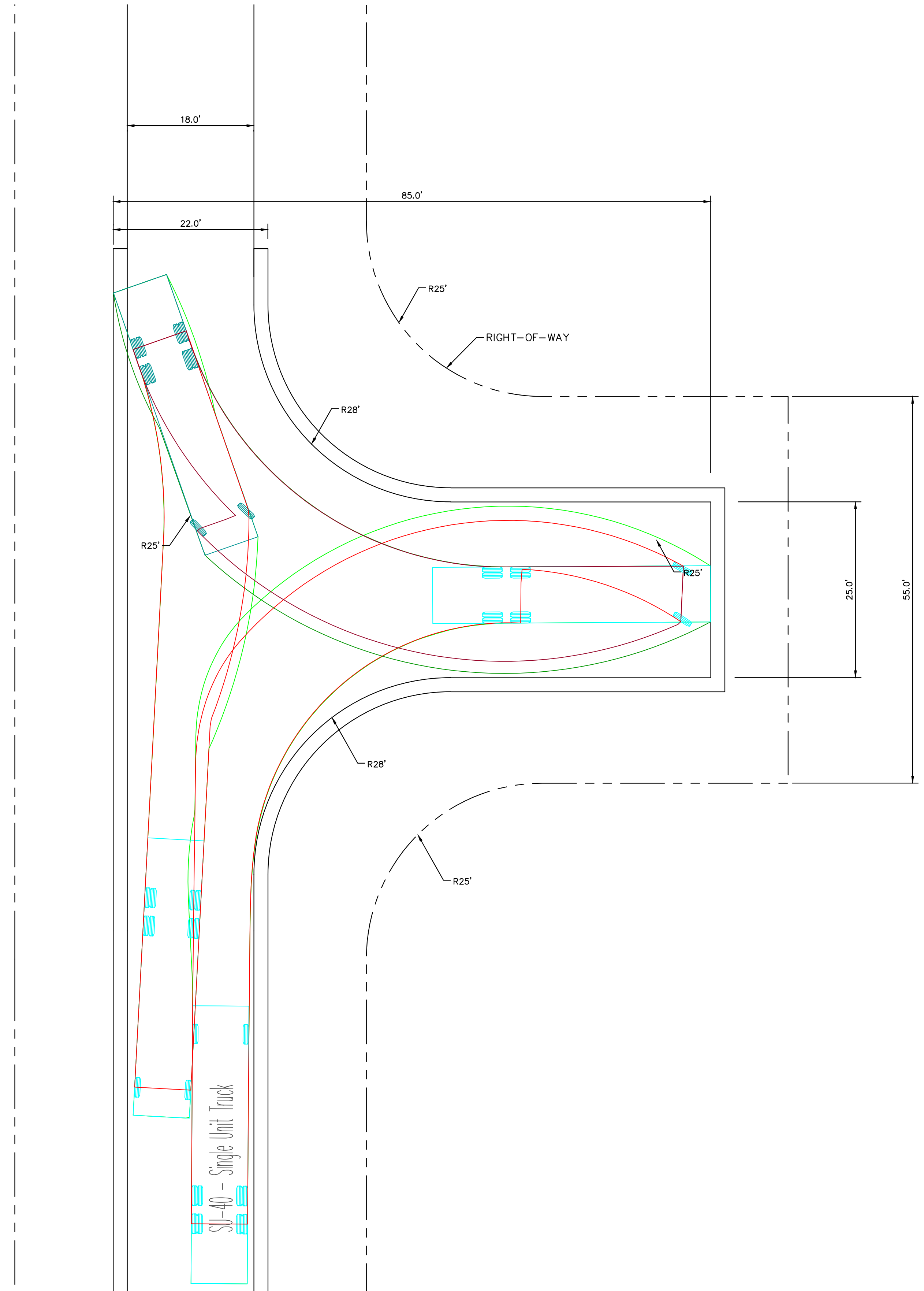
MODIFIED HAMMERHEAD
