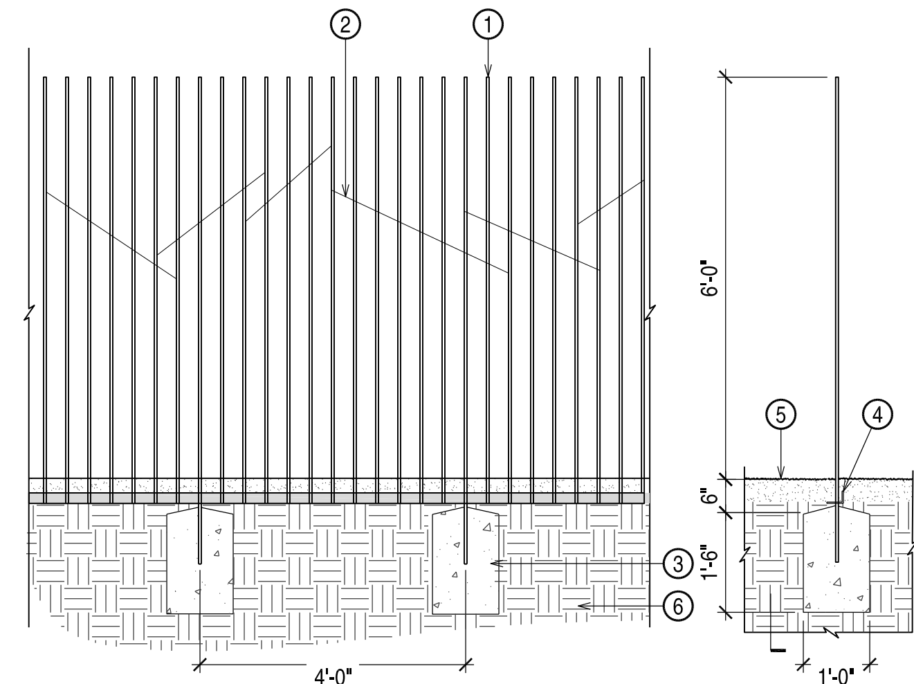
6" H STICKS IN THE DESERT FENCE SCALE: 1/2"=1'-0"
