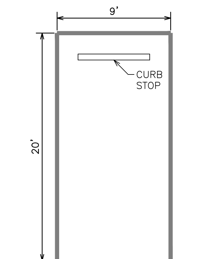
TYPICAL PARKING SPACE N.T.S.
