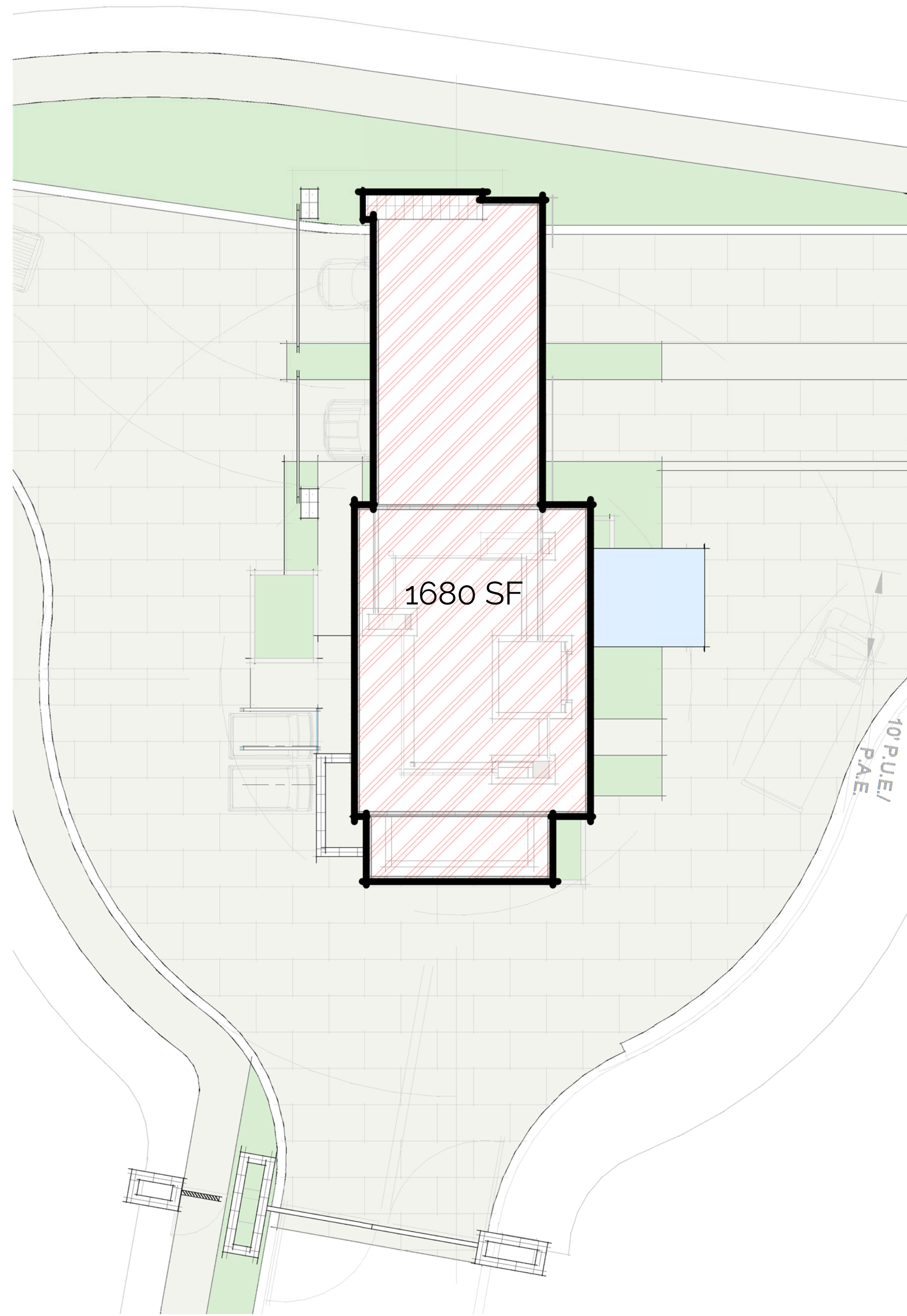
[2] ROOF DRIP LINE 1" = 10'-0"
