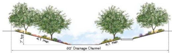
Channel Section A-A
