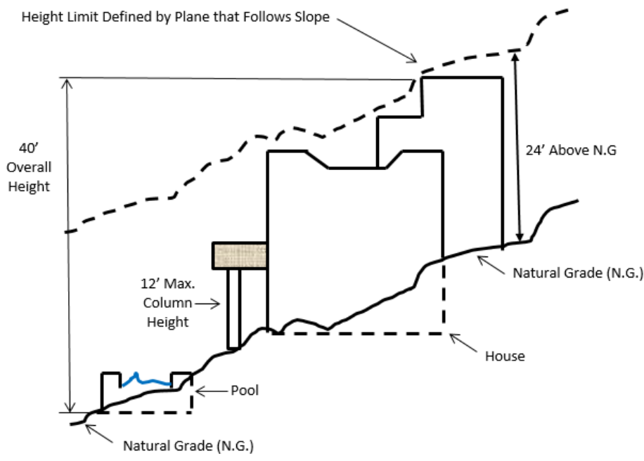
FIGURE 5 – BUILDING HEIGHT IN HILLSIDE
