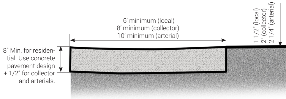
FIGURE 3.2 TYPICAL SECTION FOR VALLEY GUTTER
