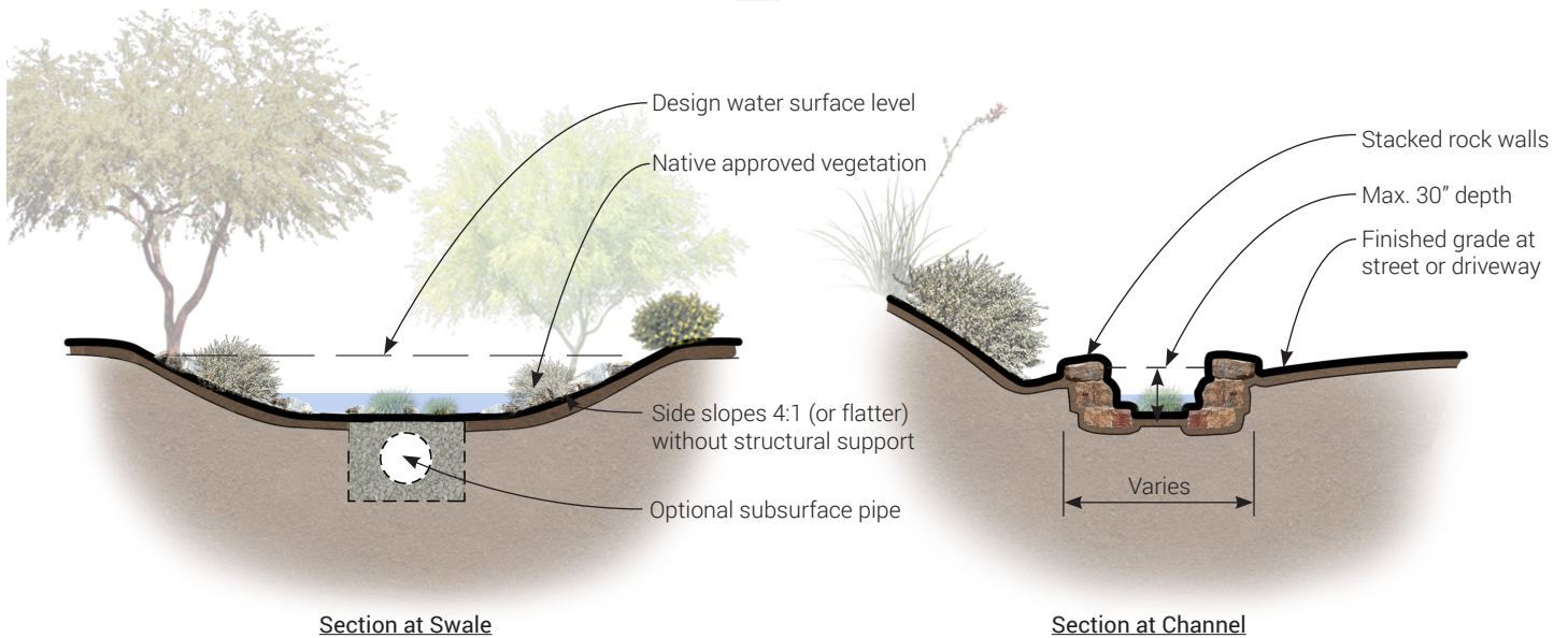
Figure 6.3 - Vegetated Swale
