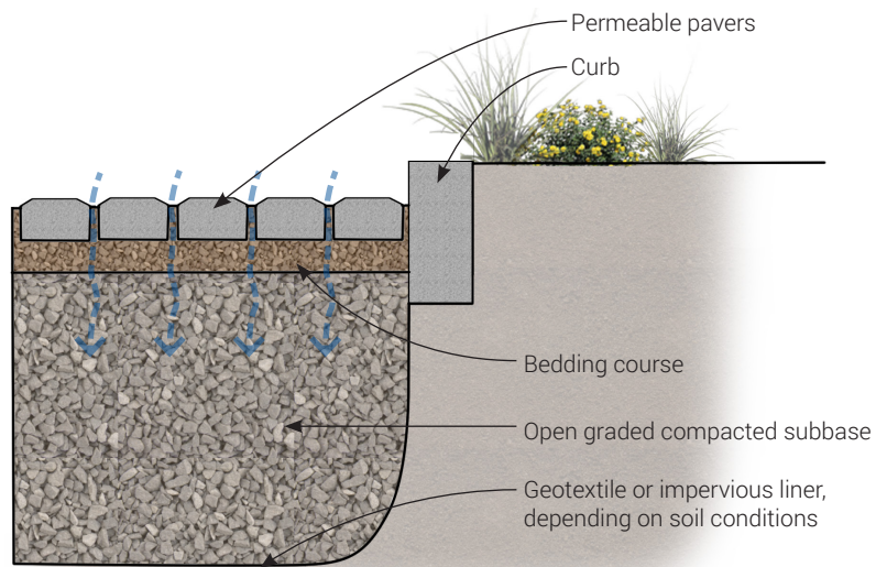
Figure 6.6 - Permeable pavers
