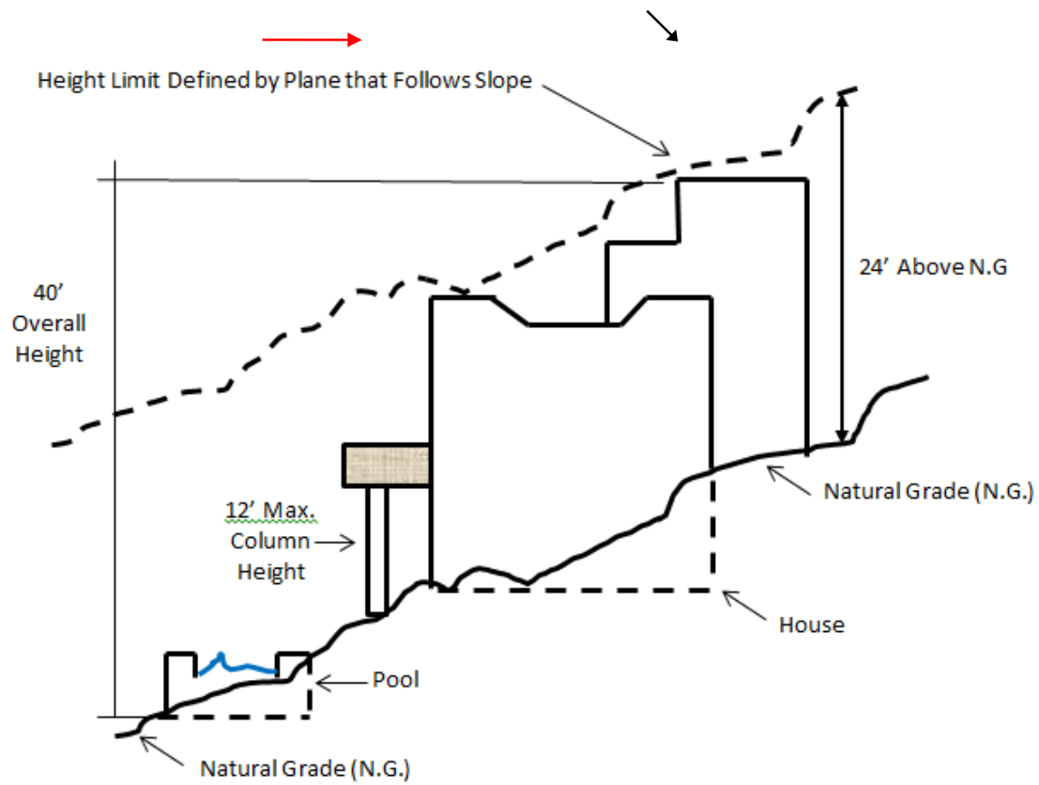
FIGURE 5 – BUILDING HEIGHT IN HILLSIDE
