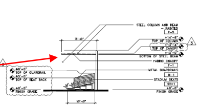
BASEBALL FIELD BLEACHER EAST/SOUTH/SOUTHEAST ELEVATION
