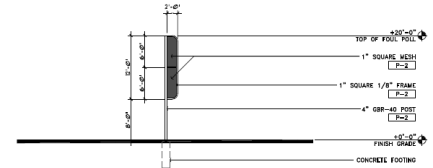
BASEBALL FIELD FOUL POLE ELEVATION - HINGED
