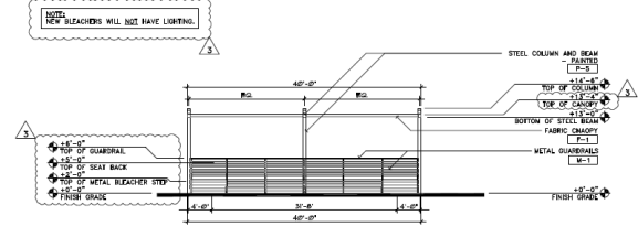
BASEBALL FIELD BLEACHER NORTH/EAST/NORTHEAST ELEVATION
