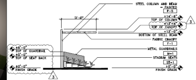
BASEBALL FIELD BLEACHER WES/NORTH/NORTHWEST ELEVATION
