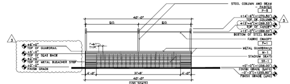
BASEBALL FIELD BLEACHER SOUTH/WEST/SOUTHWEST ELEVATION
