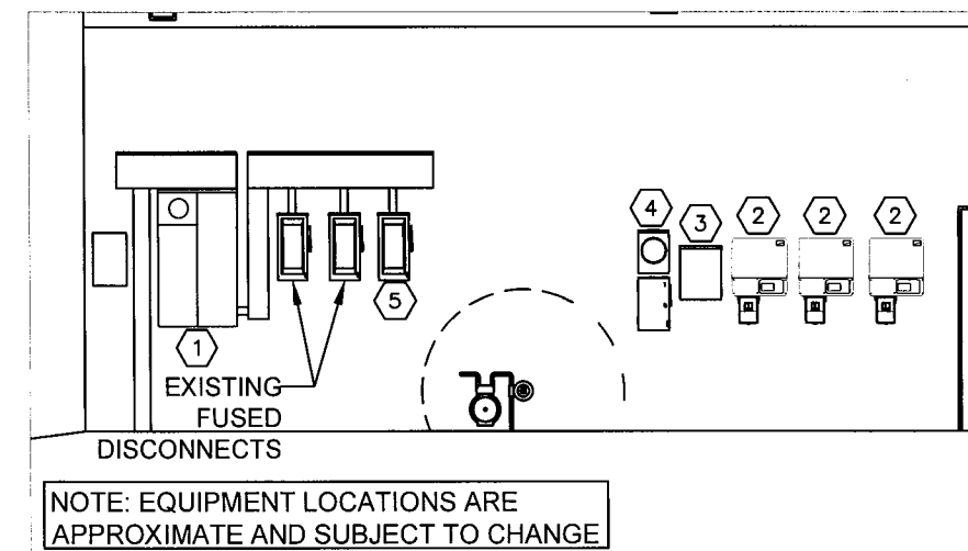
EQUIPMENT LAYOUT
