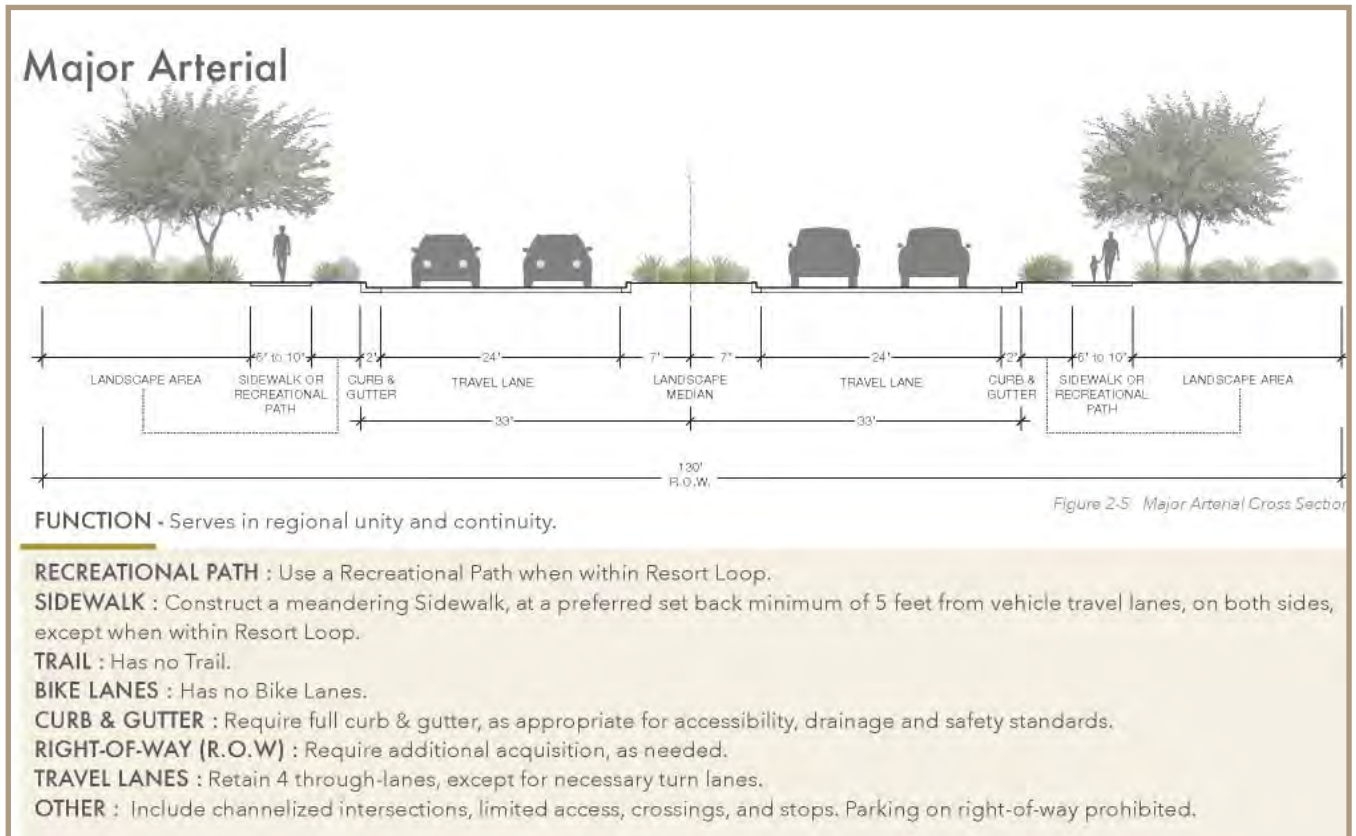
Figure 3.2: Typical Major Arterial Cross-Section, TOPV Walk & Bike Plan 2018
