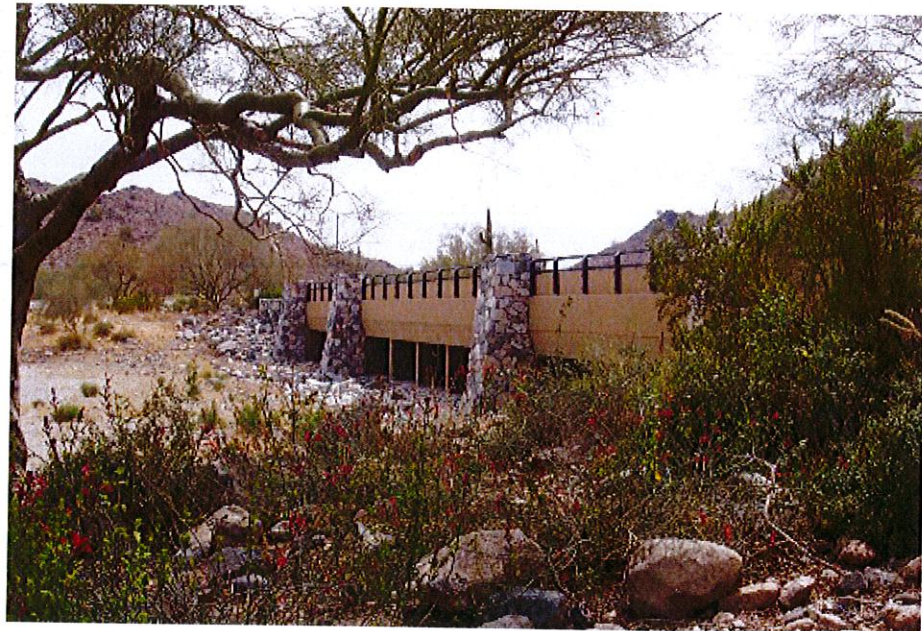
Example of Box Culvert Bridge. Wash Crossing In Parcel B to be Similar In Design.
