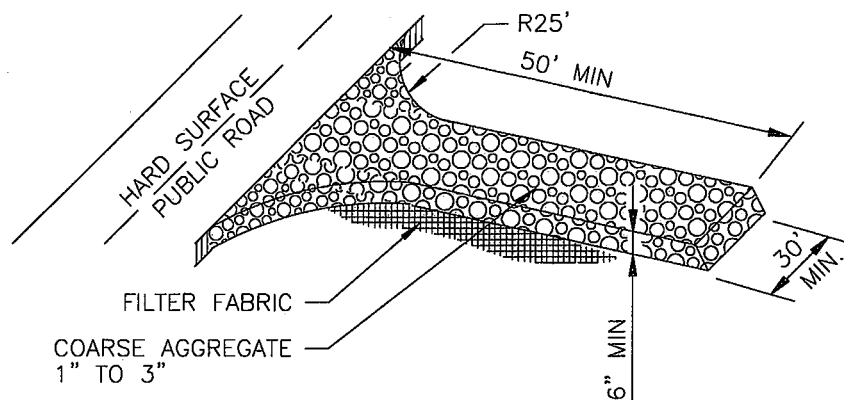
STABILIZED CONSTRUCTION ENTRANCE
