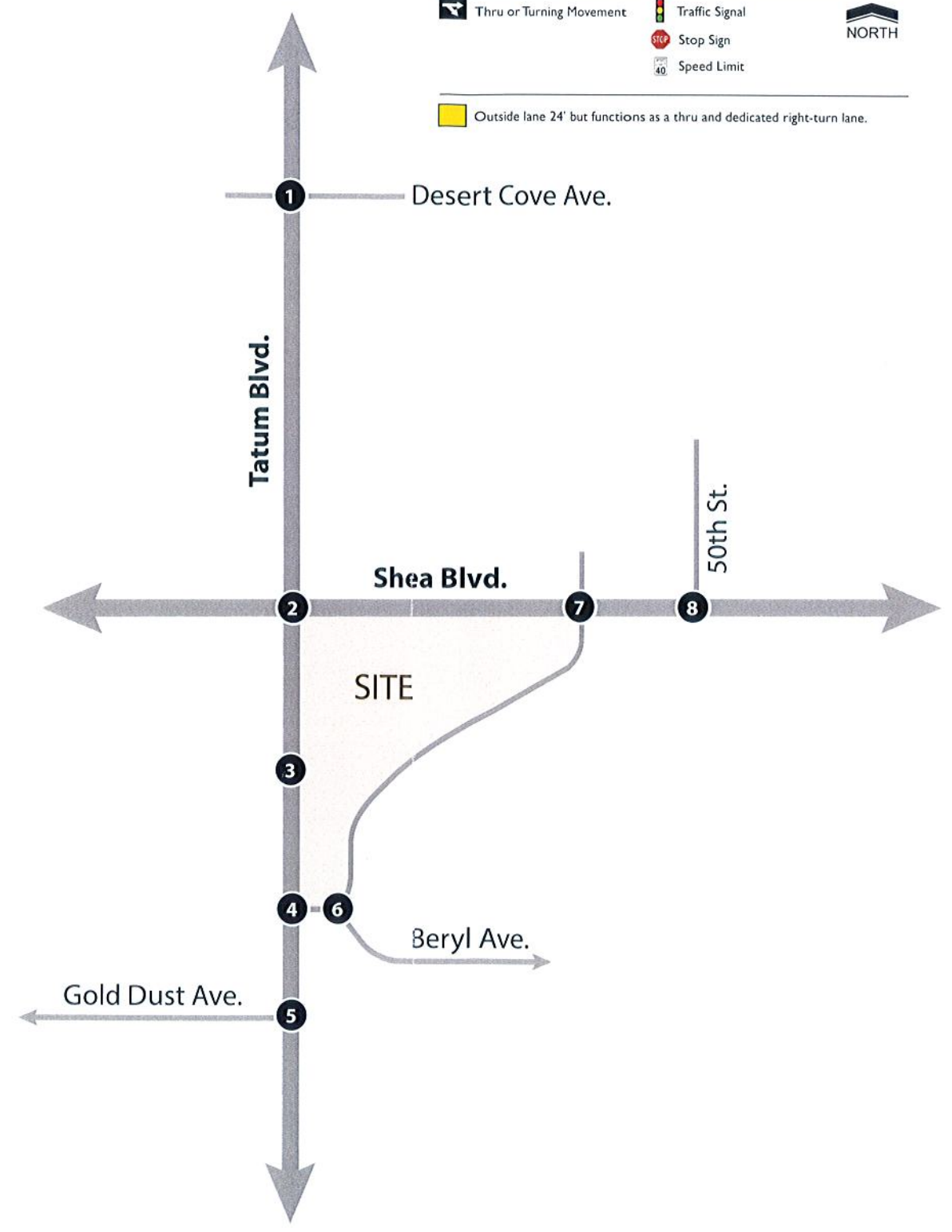
Figure 2: Existing Lane Configurations and Traffic Controls
