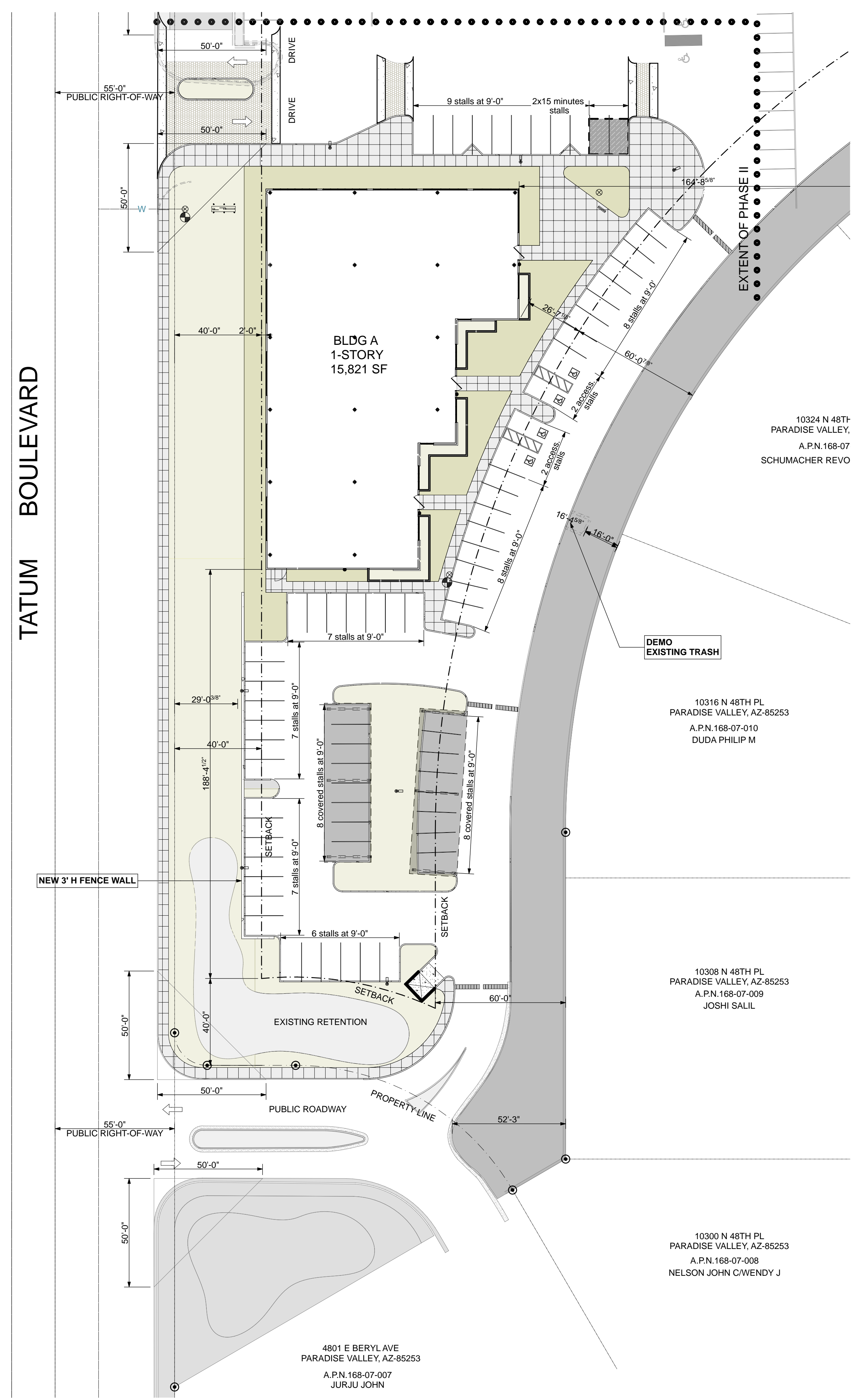
PHASE II ENLARGED PLAN
