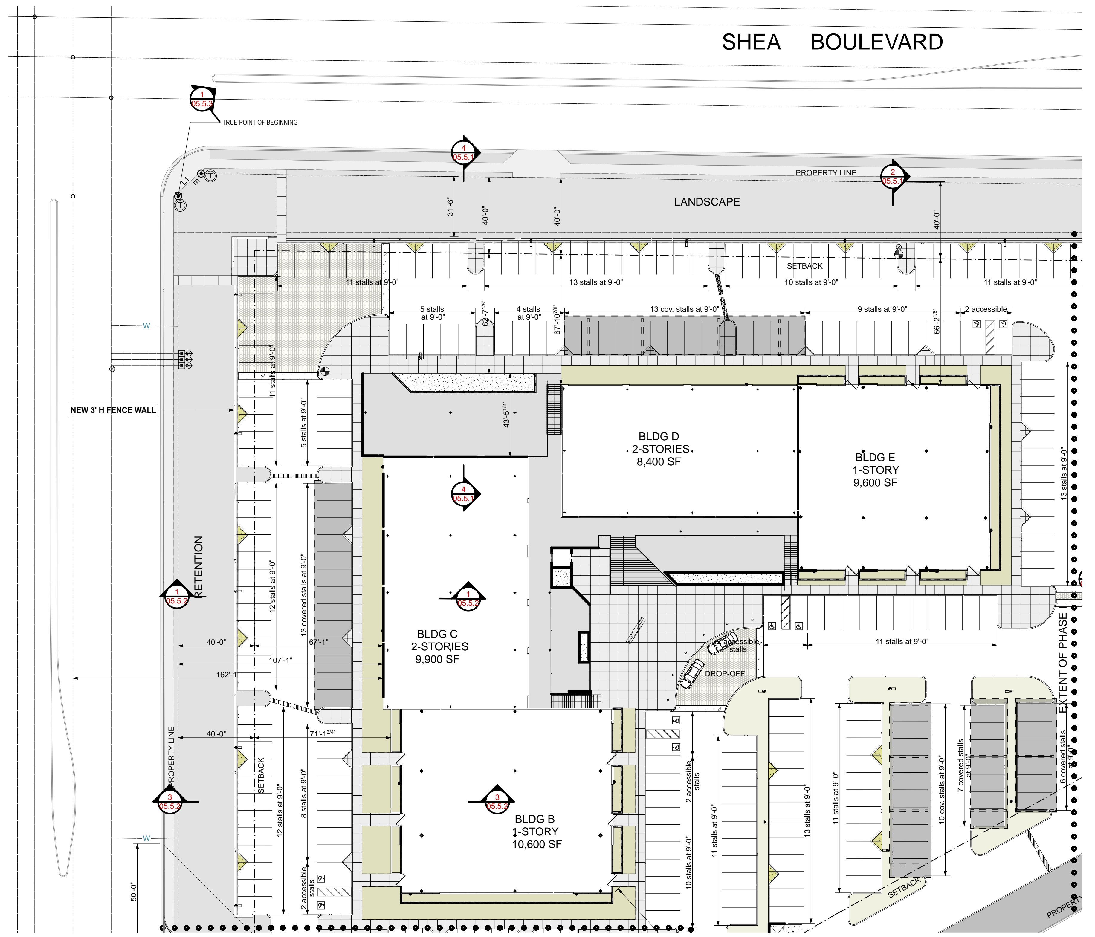
PHASE III ENLARGED PLAN 0 30' 60' NORTH
