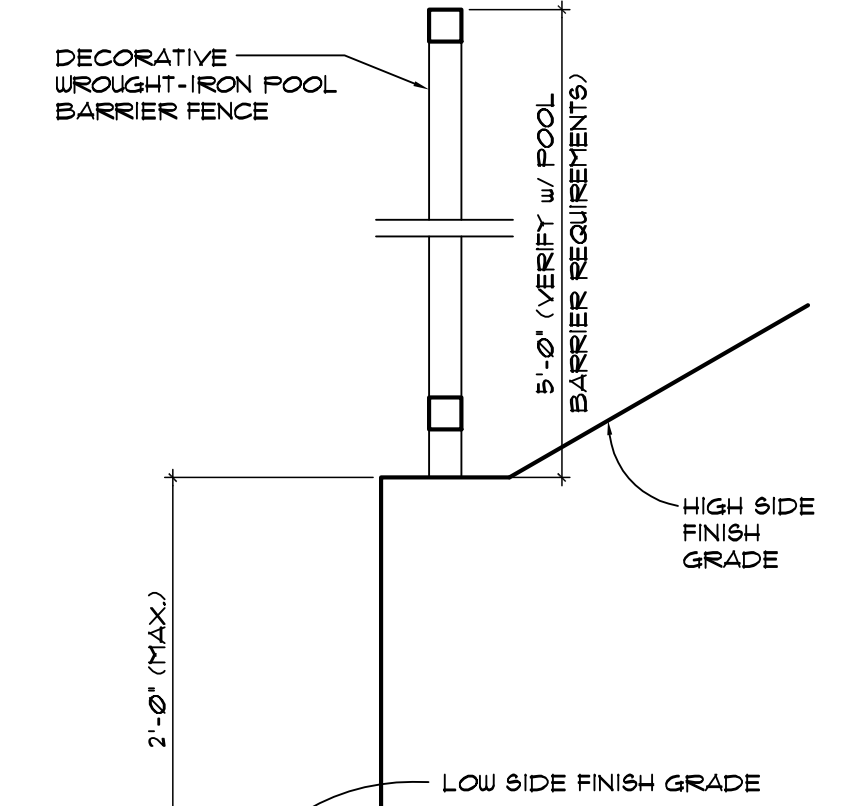
4 POOL BARRIER at HILLSIDE SCALE: 1" = 1'-0"
