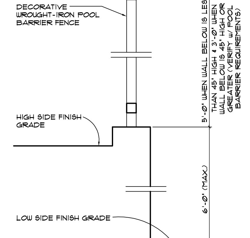
3 POOL BARRIER at RETAINING WALL SCALE: 1" = 1'-0"
