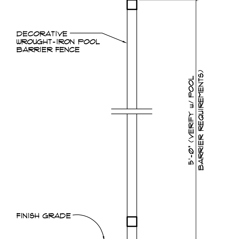
2 POOL BARRIER at FREESTANDING SCALE: 1" = 1'-0"
