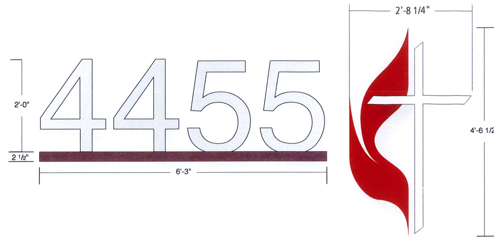
address | elevation | scale: 1/2" = 1'-0"
