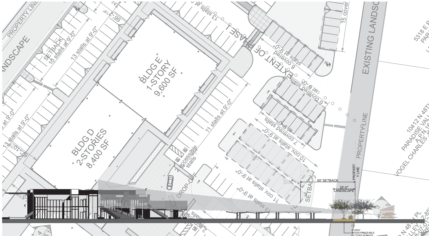
1 SECTION THROUGH BLDG E PHASE III AND ADJACENT PLOT
