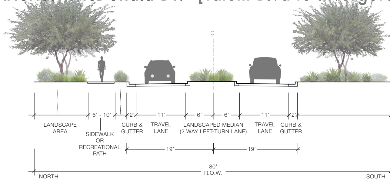
Figure 2-7 McDonald Dr. (Tatum Blvd to Invergordon Rd) Cross Section
