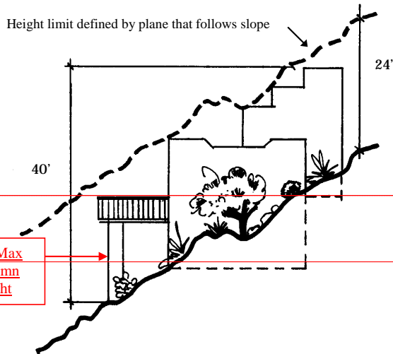
FIGURE 5 – BUILDING HEIGHT IN HILLSIDE
